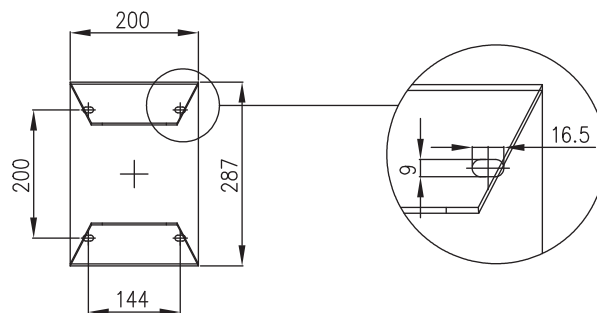
FIXING DETAILS
